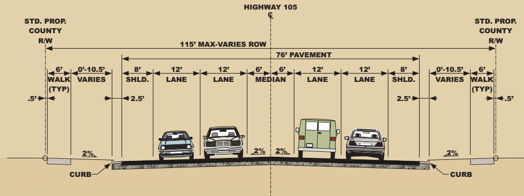
Ultimate Urban 4-Lane I-25 To Lake Woodmoor
